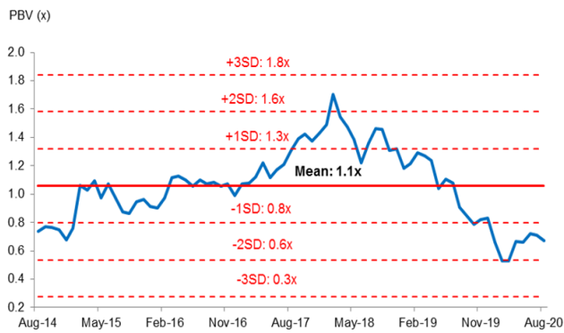
Figure 6: IRPC's forward P/BV and SD levels
