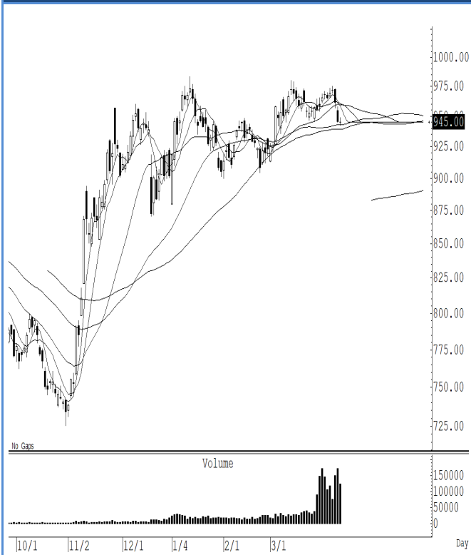
S50M21 (Close 945.00 Chg -0.50)
