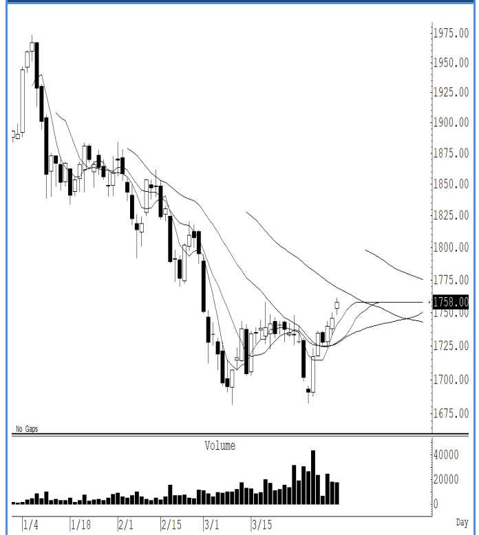
GOM21 (Close 1,758.00 Chg 12.10)
