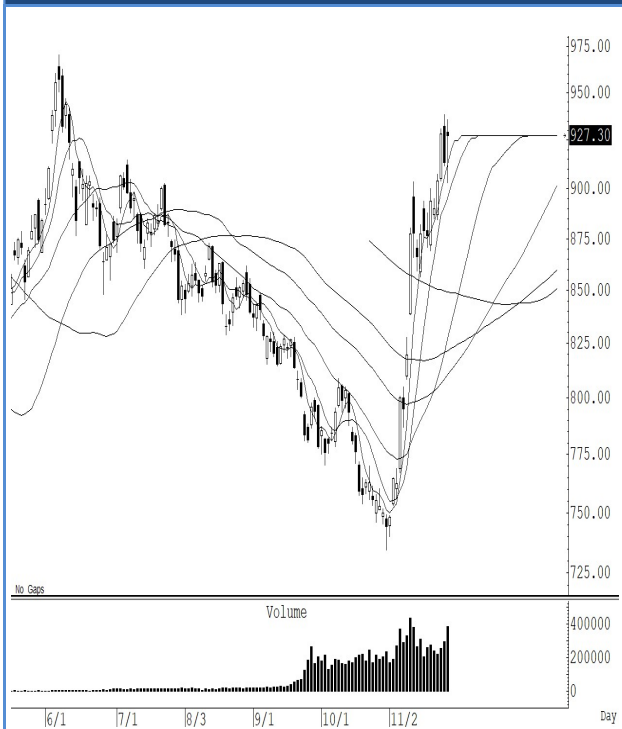
S50Z20 (Close 927.30 Chg 14.00)
