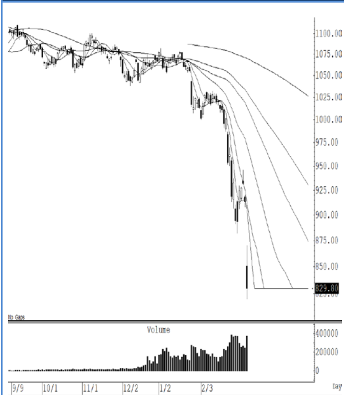
S50H20 (Close 829.80 Chg -83.90)
