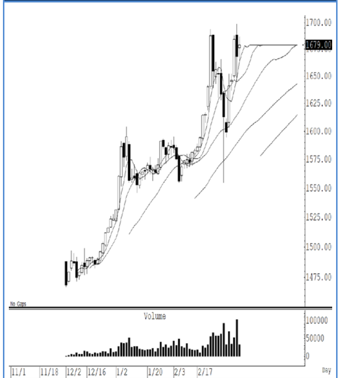
GOH20 (Close 1,679.00 Chg 11.10)
